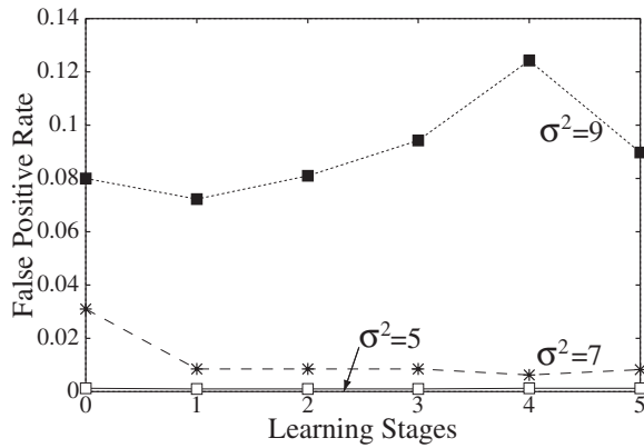
Figure 5. False-positive rate for the FP-dataset.
