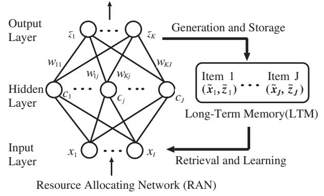
Figure 1. The architecture of RAN-LTM.
